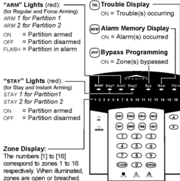
Figure 2.2: Overview of the 1689 LED Keypad
