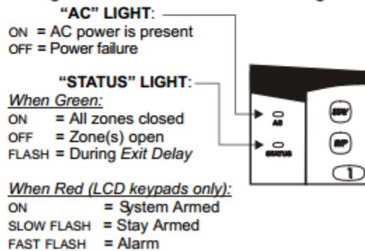
Figure 2.1: Overview of Indicator Lights
